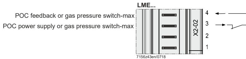
Figure 8: POC or gas pressure switch-max terminal X2-02
