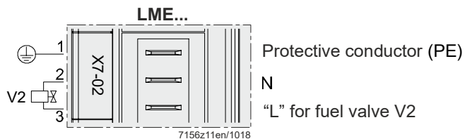
Figure 32: Fuel valve V2 terminal X7-02
