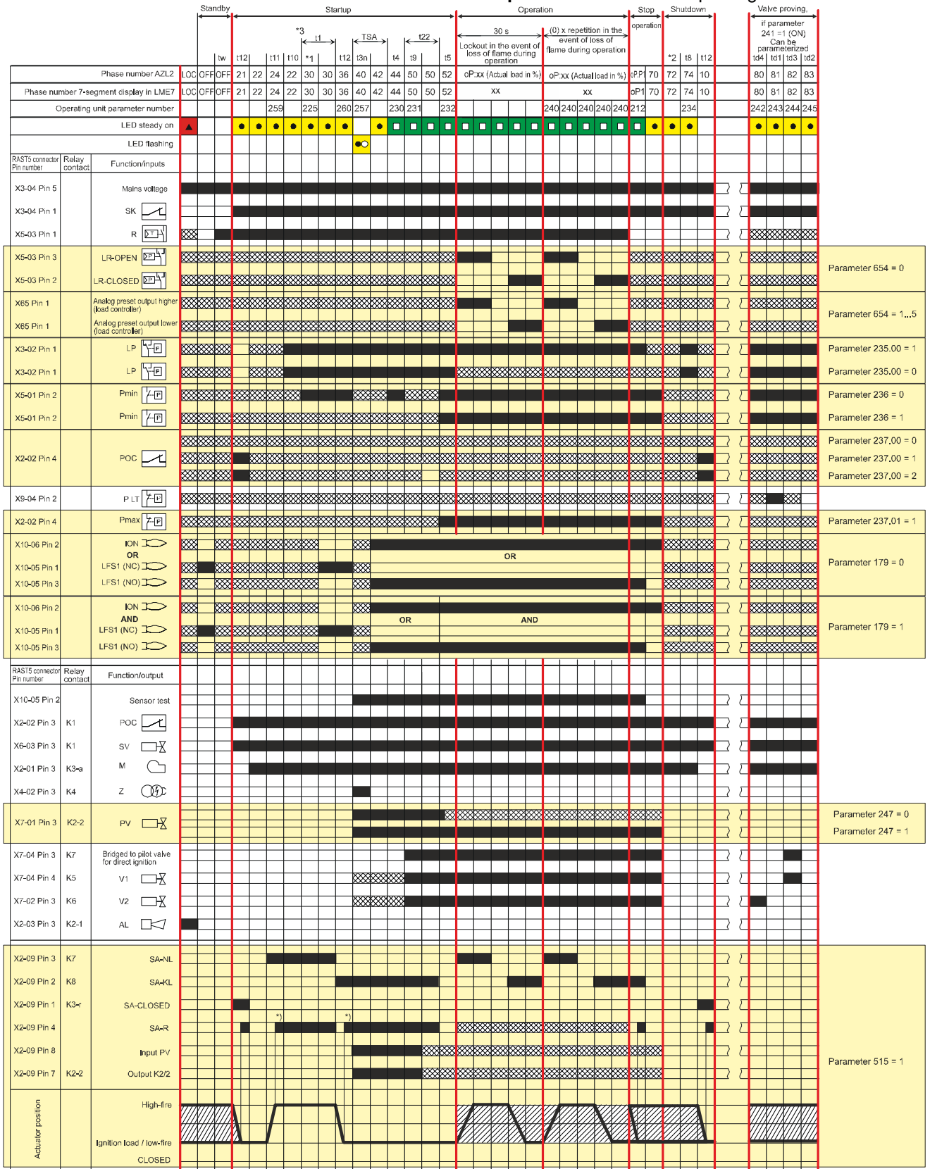
Figure 1: Program sequence for fuel trains G and Gp1 with or without valve proving
