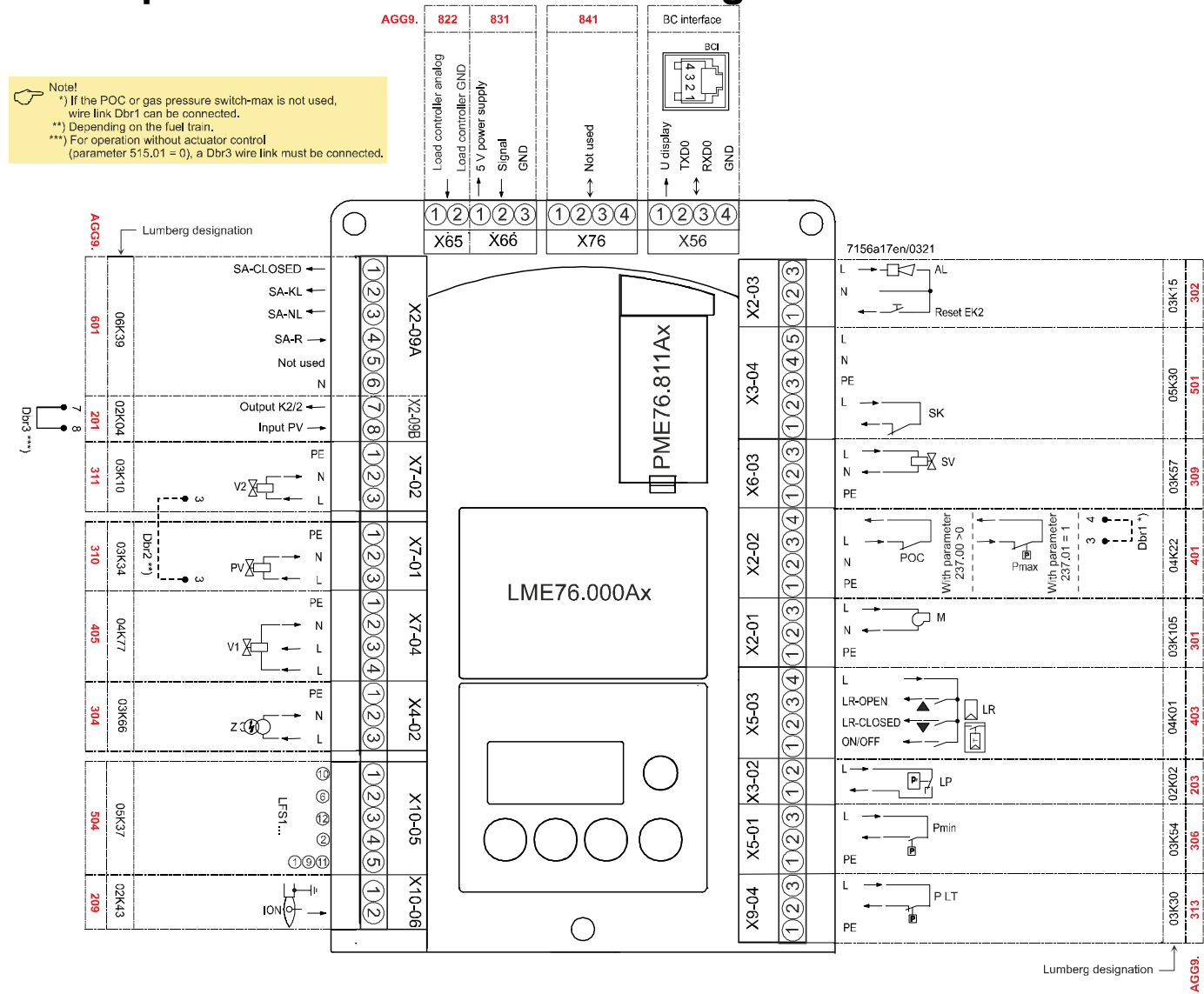
Figure 33: LME76.000Ax: Inputs and outputs / internal connection diagram
