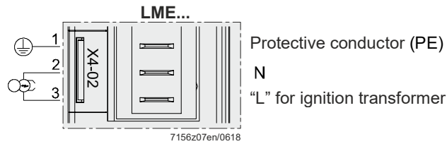
Figure 28: Ignition transformer terminal X4-02
