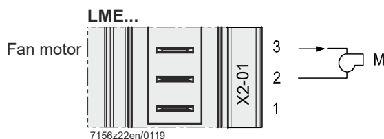
Figure 20: Fan motor terminal X2-01
