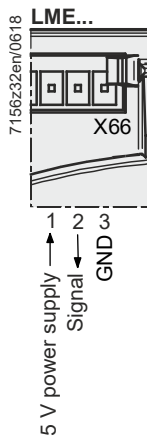
Figure 23: Actuator terminal X66
