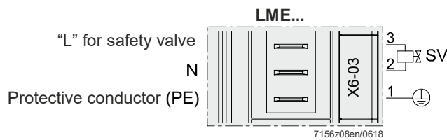
Figure 29: Safety valve terminal X6-03
