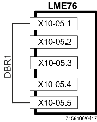
Figure 13: Connection diagram of an ionization probe only without LFS1
