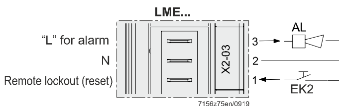
Figure 217: Alarm / remote lockout reset terminal X2-03
