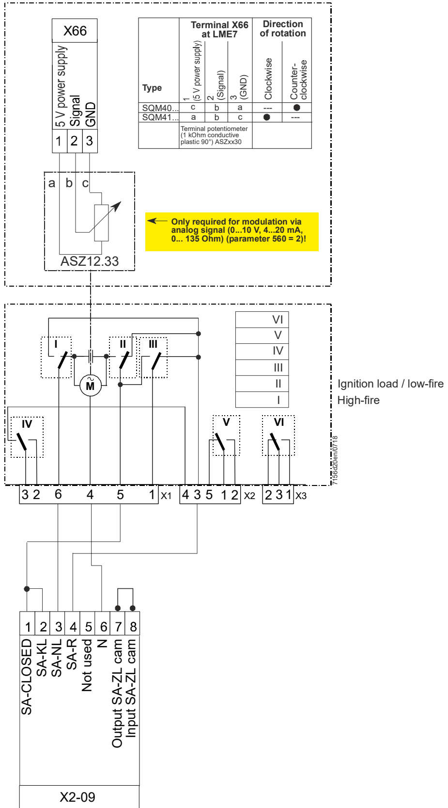
Figure 26: Connection diagram example 1: LME76.000Ax with SQM40/SQM41 (Diagram 8) and ASZ
