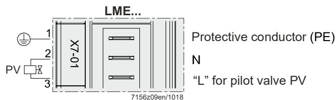
Figure 30: Pilot valve PV terminal X7-01
