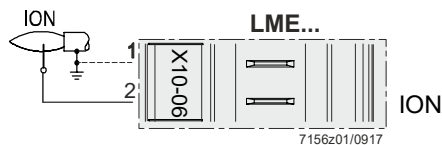
Figure 11: Ionization probe terminal X10-06
