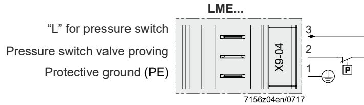
Figure 9: Pressure switch valve proving terminal X9-04
