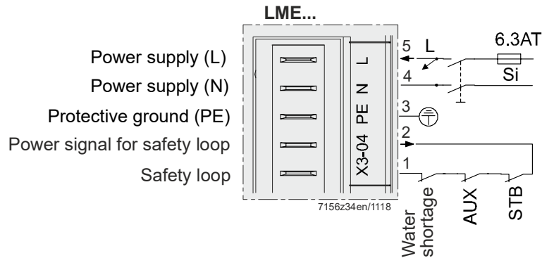
Figure 19: Safety loop terminal X3-04
