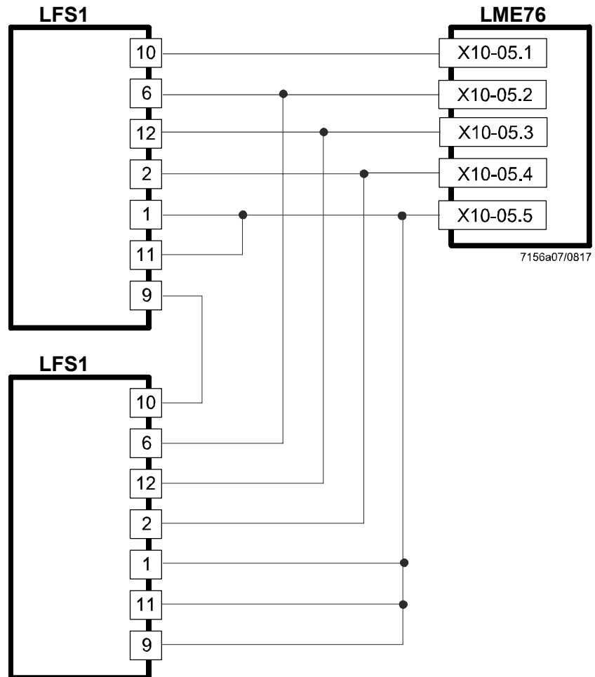
Figure 15: Connection diagram with 2x LFS1 in logical OR operation
