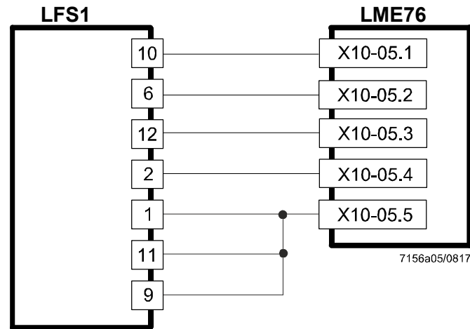
Figure 14: Connection diagram with LFS1
