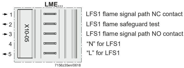
Figure 12: LFS1 terminal X10-05
