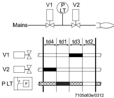
Figure 10: Valve proving with separate pressure switch
