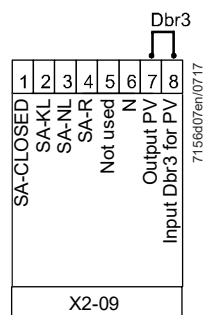
Figure 27: Connection diagram example 2: LME76.000Ax with PME76.811Ax without actuator
