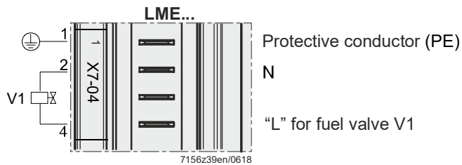
Figure 31: Fuel valve V1 terminal X7-04
