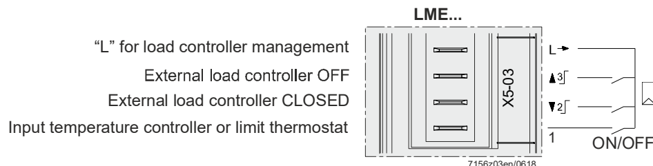
Figure 18: Load controller ON/OFF terminal X5-03
