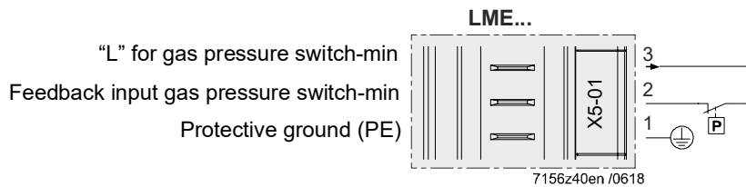
Figure 7: Gas pressure switch-min terminal X5-01
