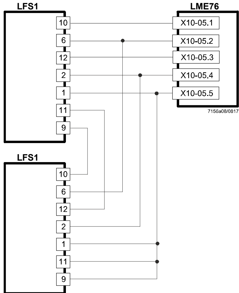
Figure 16: Connection diagram with 2x LFS1 in logical AND operation
