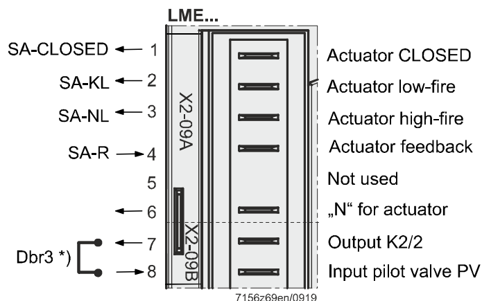
Figure 22: Actuator terminal X2-09
