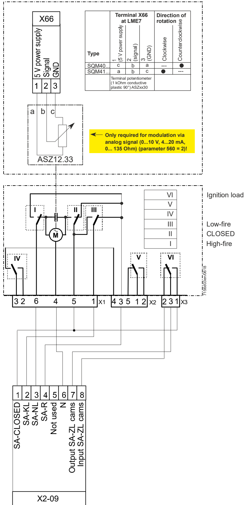
Figure 26: Connection diagram example 1: LME75.000Ax with SQM40/SQM41 (diagram 8) and ASZ
