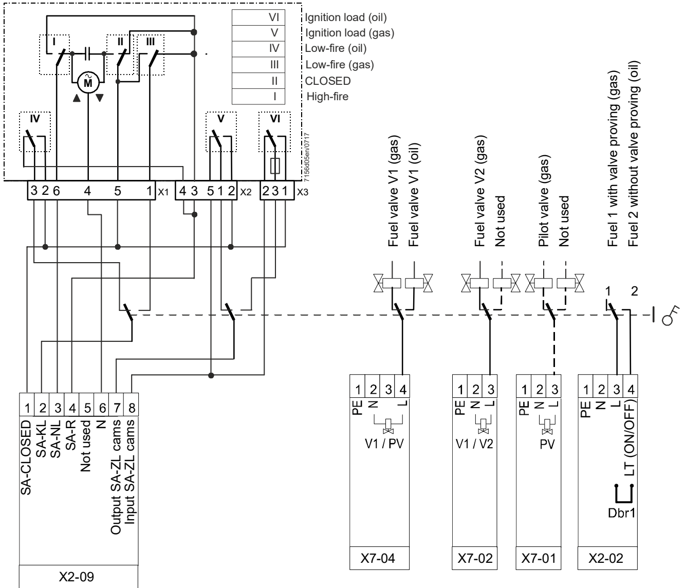
Figure 31: Connection diagram example 3: LME75.000Ax with SQM40/SQM41, oil/gas fuel modulating
