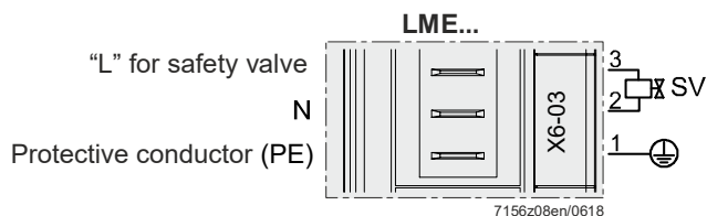
Figure 36: Safety valve terminal X6-03
