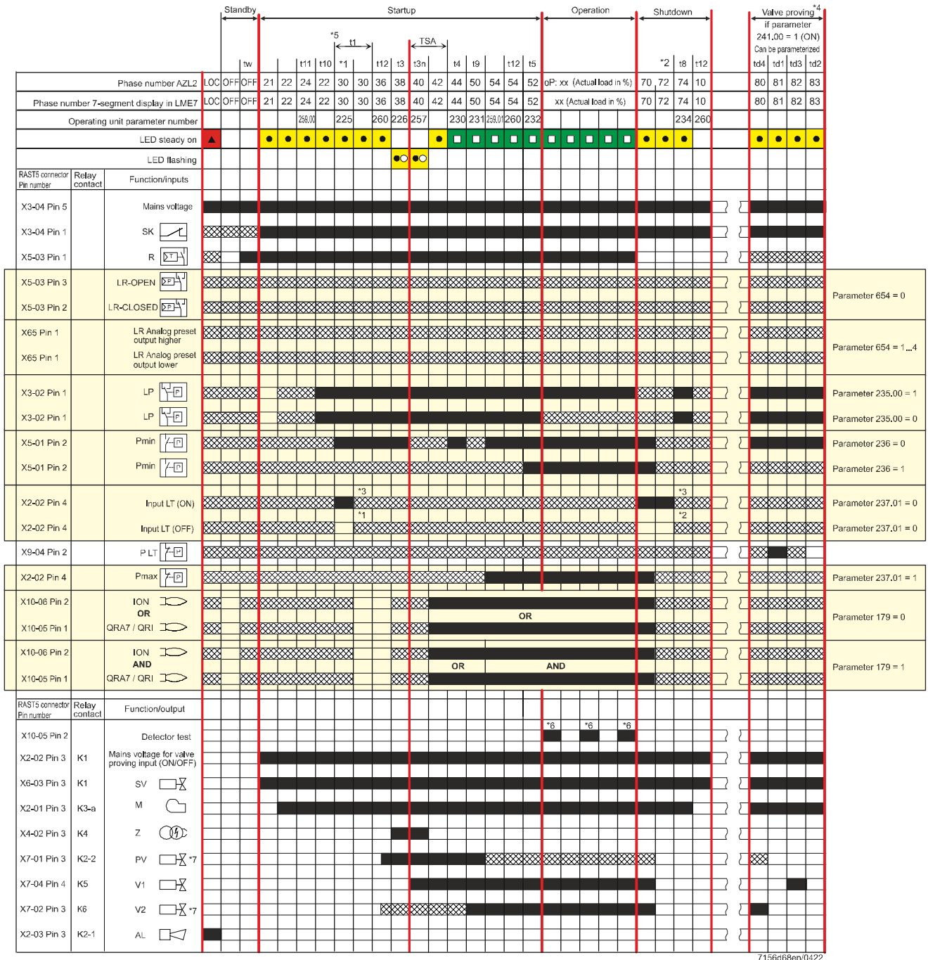
Figure 5: Program sequence for fuel trains G without/with valve proving, Gp1 with valve proving, and Gp2 without valve proving
