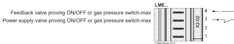
Figure 12: Gas pressure switch-max or valve proving terminal X2-02
