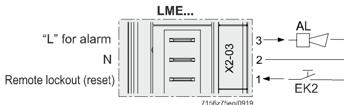
Figure 21: Alarm / remote lockout reset terminal X2-03
