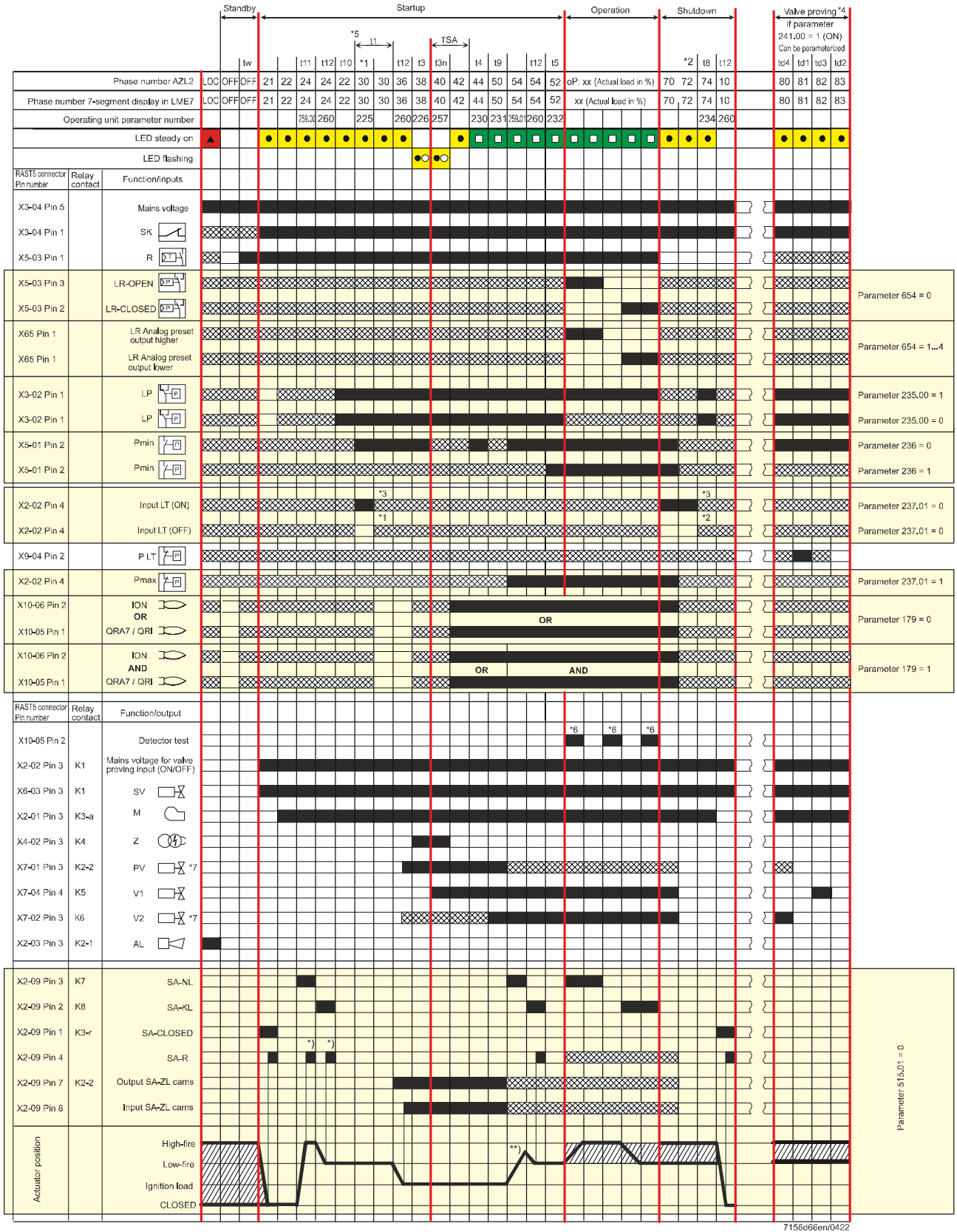
Figure 3: Program sequence for fuel trains G without/with valve proving, Gp1 with valve proving, and Gp2 without valve proving
