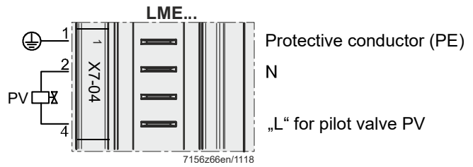
Figure 38: Pilot valve PV terminal X7-04
