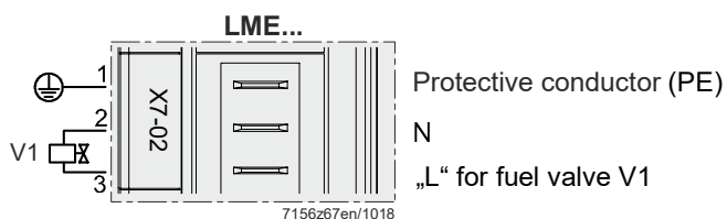
Figure 39: Fuel valve V1 terminal X7-02
