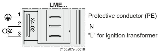
Figure 35: Ignition transformer terminal X4-02
