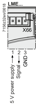
Figure 23: Actuator terminal X66
