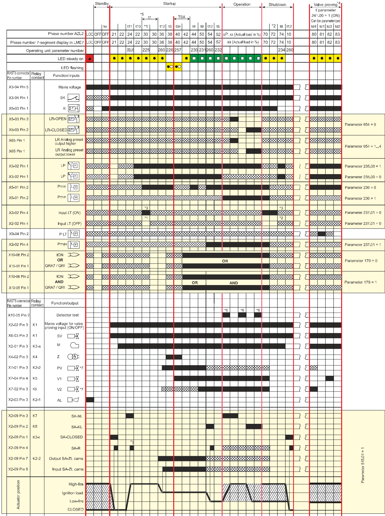
Figure 2: Program sequence for fuel trains G without/with valve proving, Gp1 with valve proving, and Gp2 without valve proving
