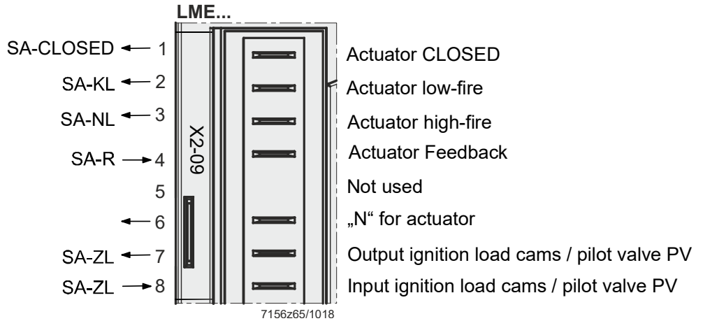
Figure 22: Actuator terminal X2-09
