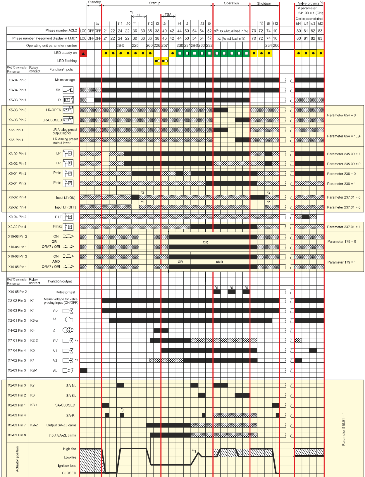
Figure 1: Program sequence for fuel trains G without/with valve proving, Gp1 with valve proving, and Gp2 without valve proving
