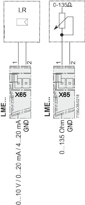
Figure 17: Load controller terminal X65
