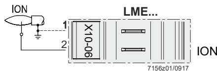
Figure 15: Ionization probe terminal X10-06
