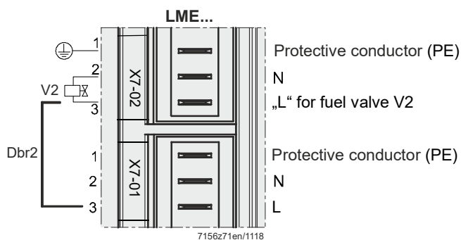
Figure 41: Fuel valve V2 terminal X7-01
