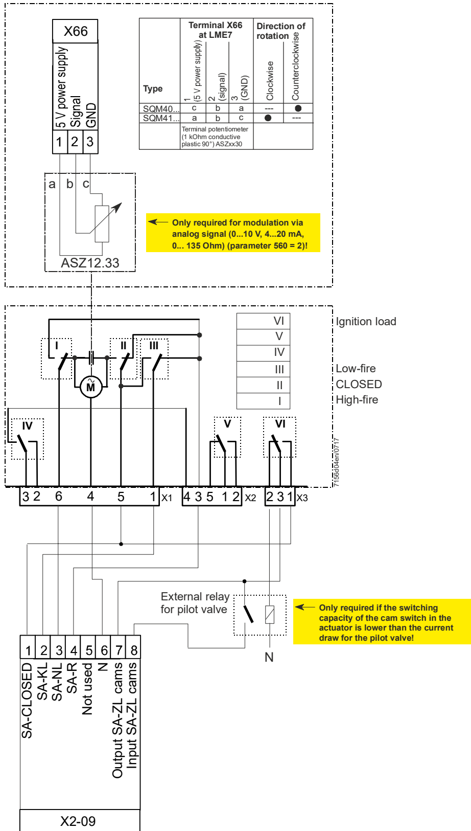
Figure 29: Connection diagram example 2: LME75.000Ax with SQM40/SQM41 (diagram 8) with external relay for pilot valve
