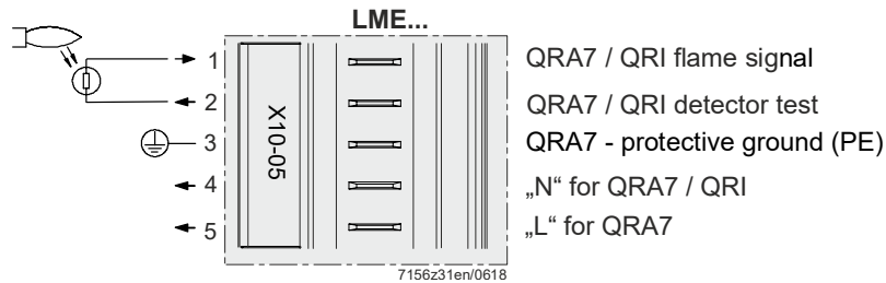
Figure 16: QRA7 / QRI terminal X10-05
