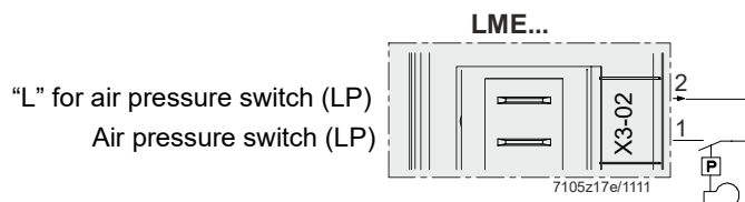
Figure 10: Air pressure switch terminal X3-02
