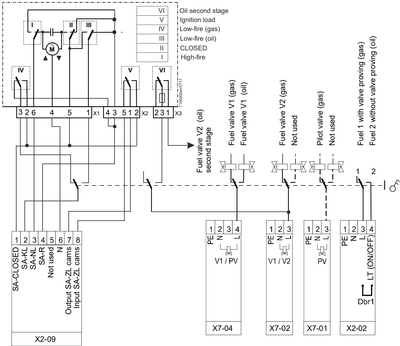
Figure 33: Connection diagram example 4: LME75.000Ax with SQM40/SQM41 gas fuel modulating, oil 2-stage
