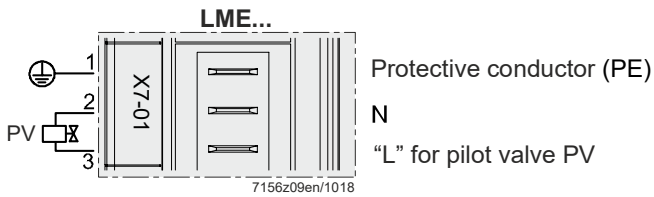
Figure 37: Pilot valve PV terminal X7-01
