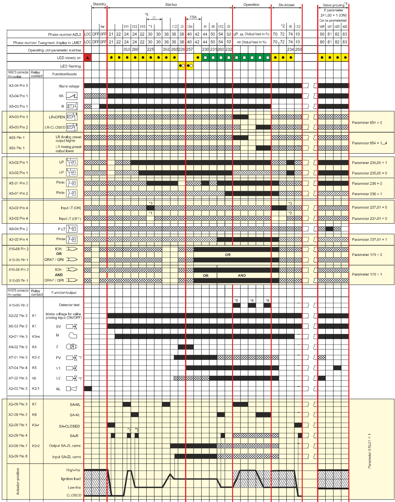
Figure 4: Program sequence for fuel trains G without/with valve proving, Gp1 with valve proving, and Gp2 without valve proving
