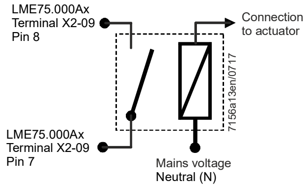
Figure 28: External relay connection diagram
