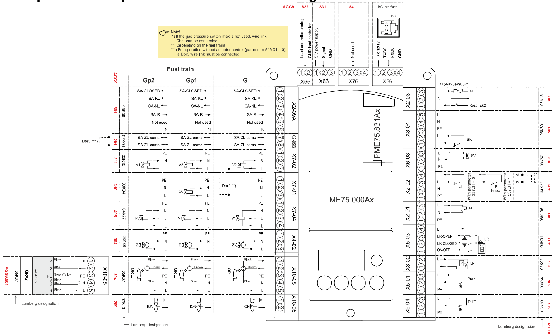
Figure 43: LME75.000Ax: Inputs and outputs/internal connection diagram
