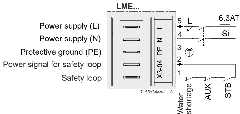
Figure 13: Safety loop terminal X3-04
