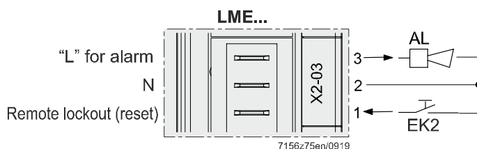
Figure 15: Alarm / remote lockout reset terminal X2-03
