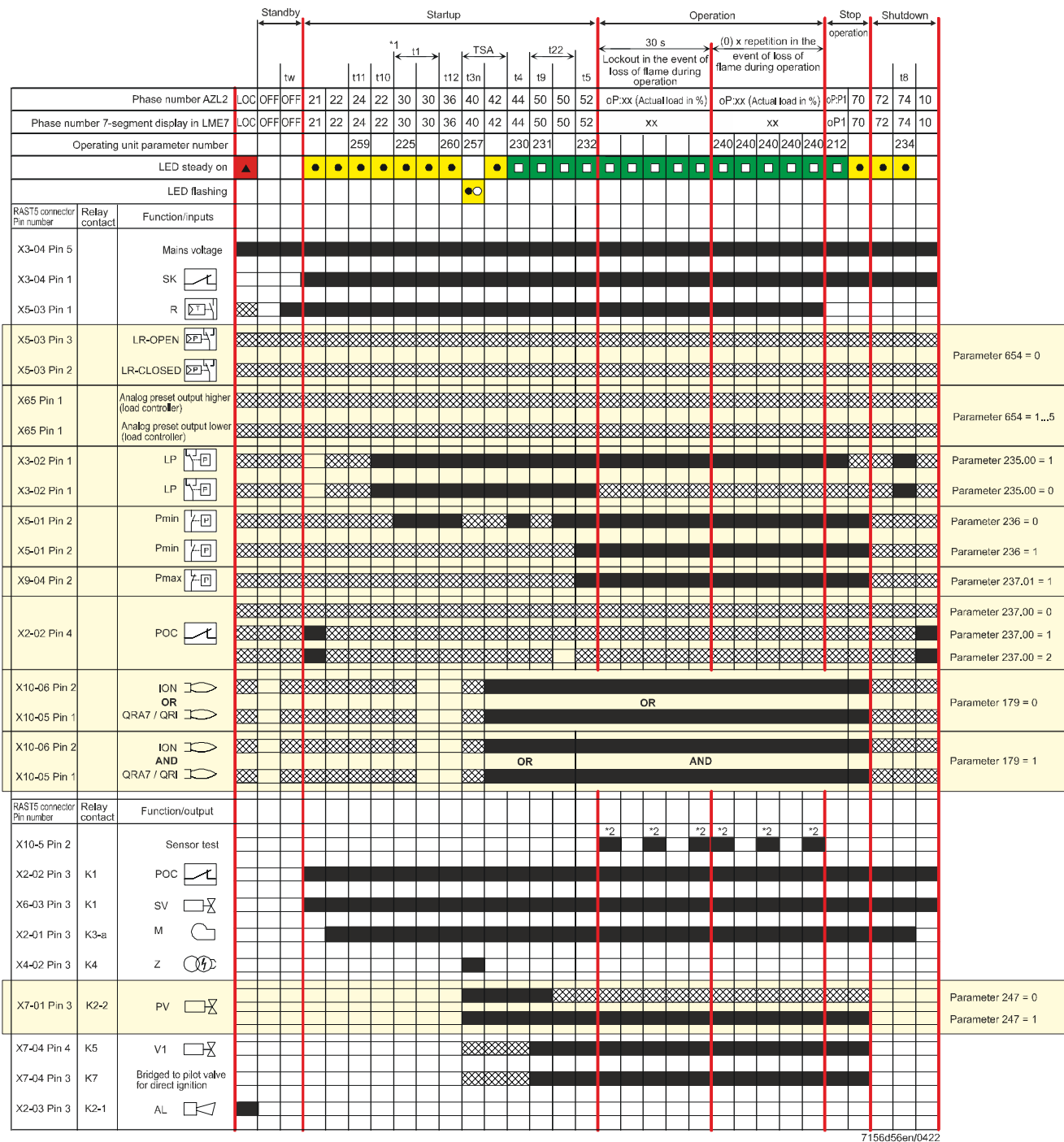
Figure 2: Program sequence for fuel trains G and Gp1/1
