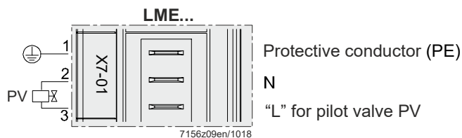
Figure 24: Pilot valve PV terminal X7-01
