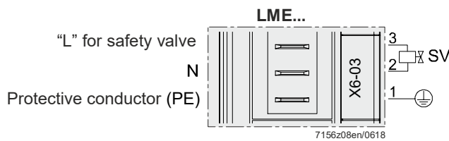
Figure 23: Safety valve terminal X6-03
