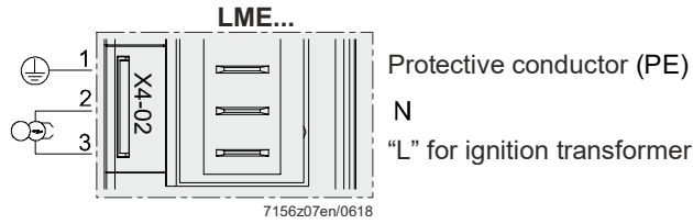
Figure 22: Ignition transformer terminal X4-02
