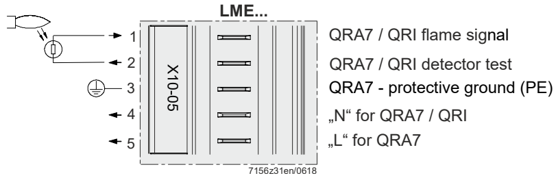
Figure 10: QRA7/QRI terminal X10-05
