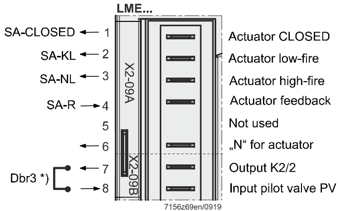
Figure 16: Actuator terminal X2-09
