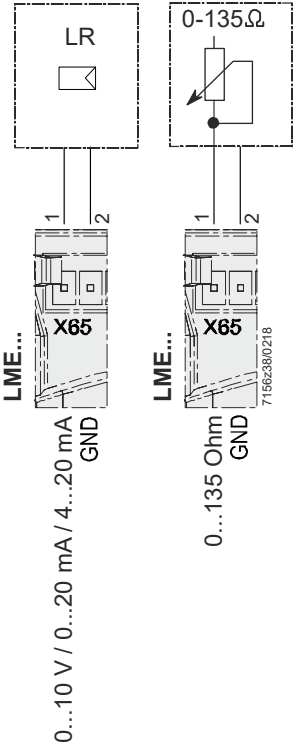
Figure 11: Load controller terminal X65
