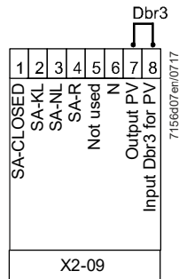
Figure 21: Connection diagram example 2: LME75.000Ax with PME75.812Ax without actuator
