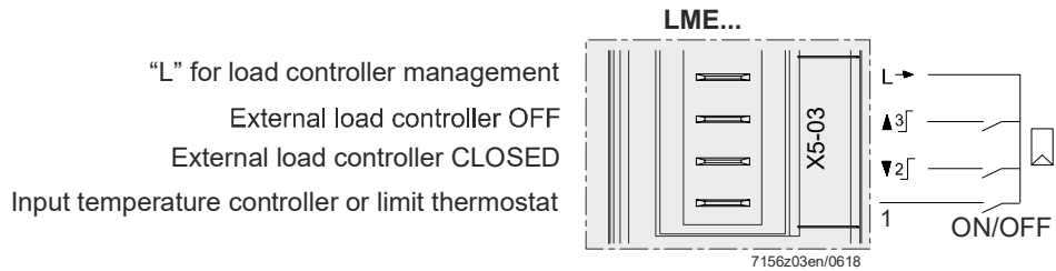
Figure 12: Load controller ON/OFF terminal X5-03
