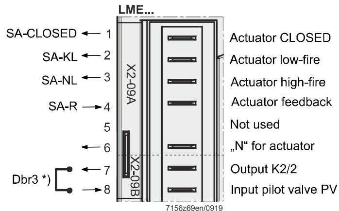
Figure 18: Actuator terminal X2-09
