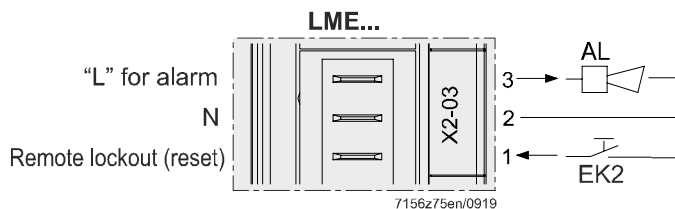
Figure 177: Alarm / remote lockout reset terminal X2-03
