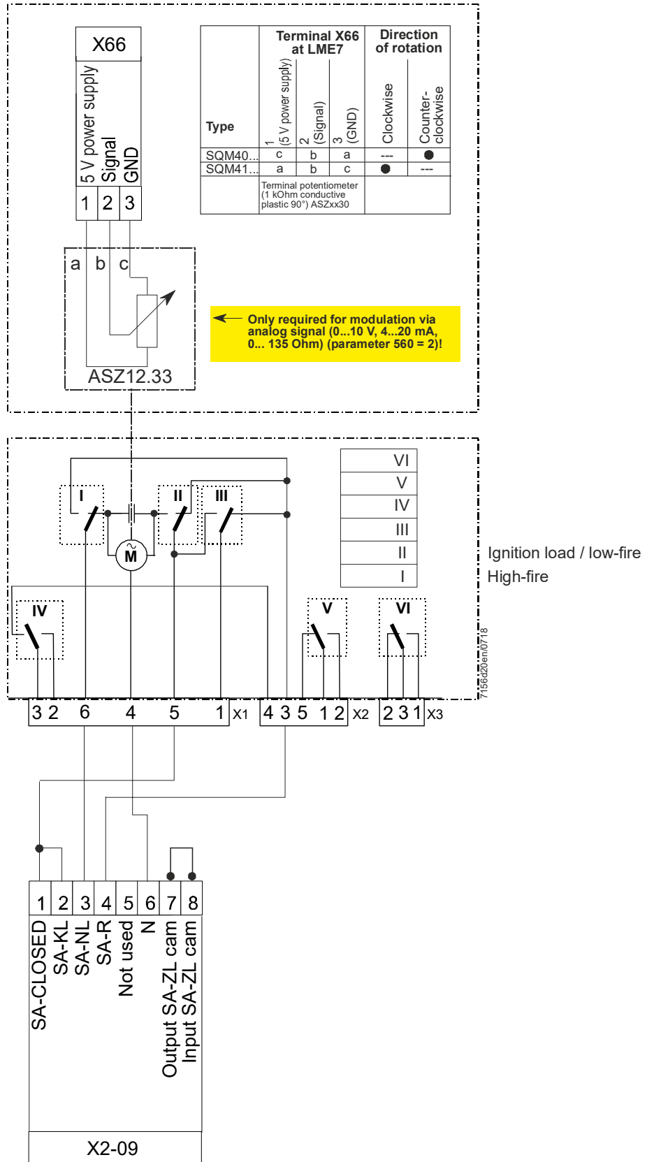
Figure 22: Connection diagram example 1: LME75.000Ax with SQM40/SQM41 (diagram 8) and ASZ
