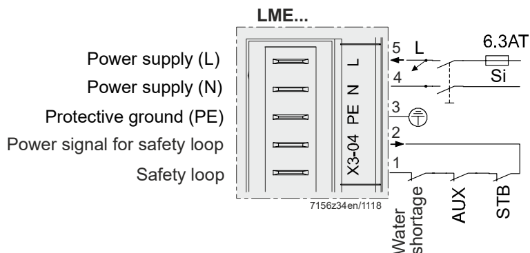
Figure 15: Safety loop terminal X3-04
