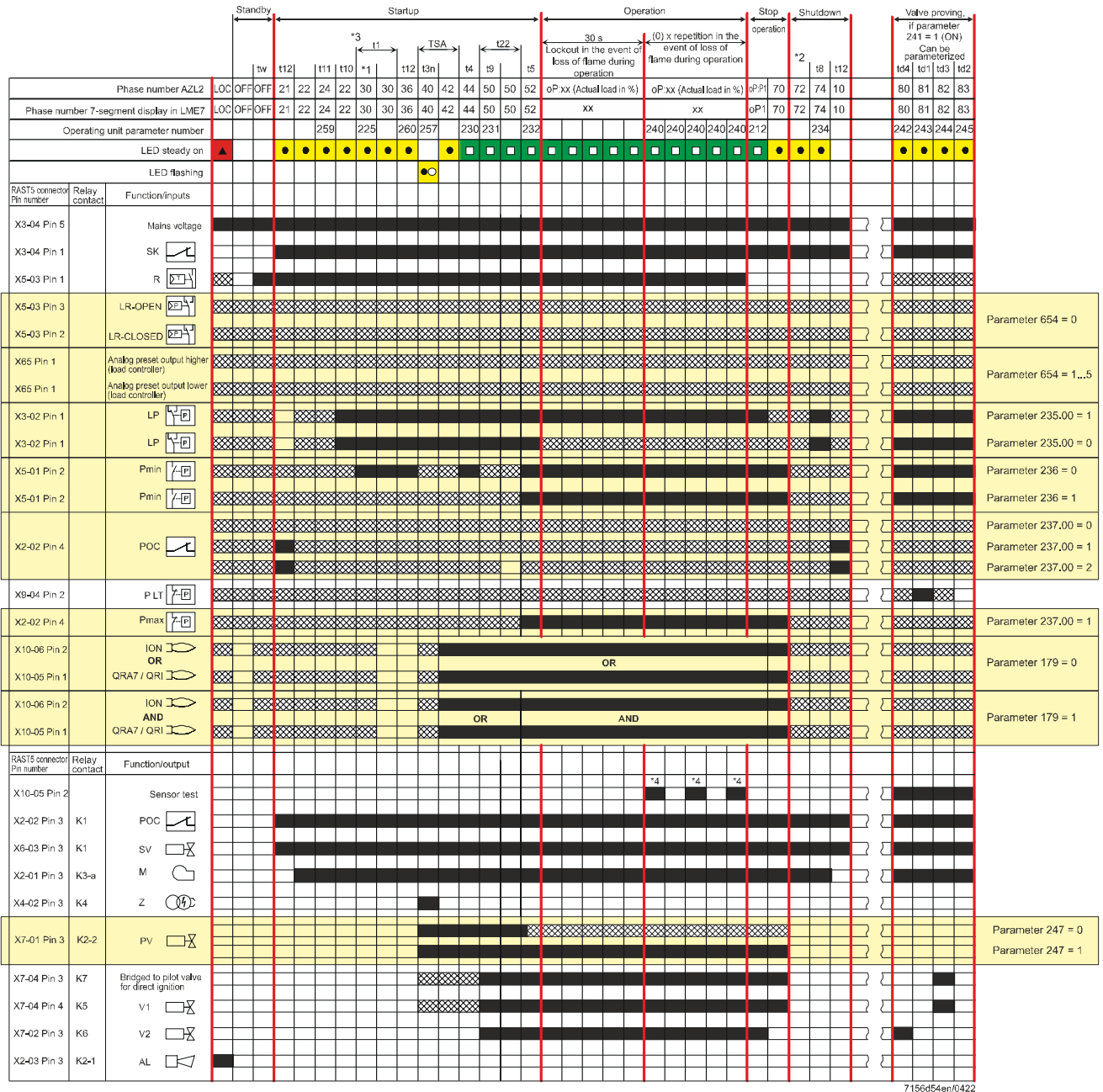
Figure 2: Program sequence for fuel trains G and Gp1 with or without valve proving
