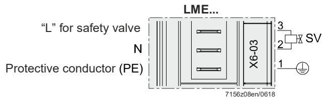
Figure 25: Safety valve terminal X6-03
