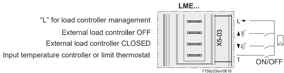
Figure 14: Load controller ON/OFF terminal X5-03
