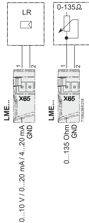
Figure 13: Load controller terminal X65
