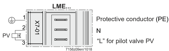
Figure 26: Pilot valve PV terminal X7-01
