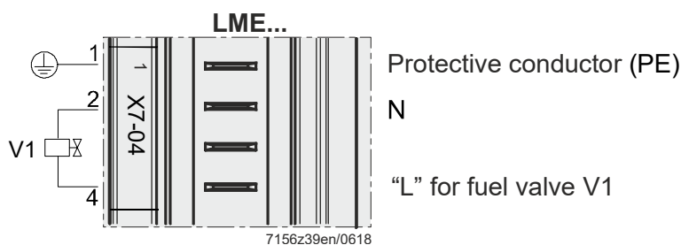
Figure 27: Fuel valve V1 terminal X7-04
