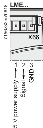
Figure 19: Actuator terminal X66
