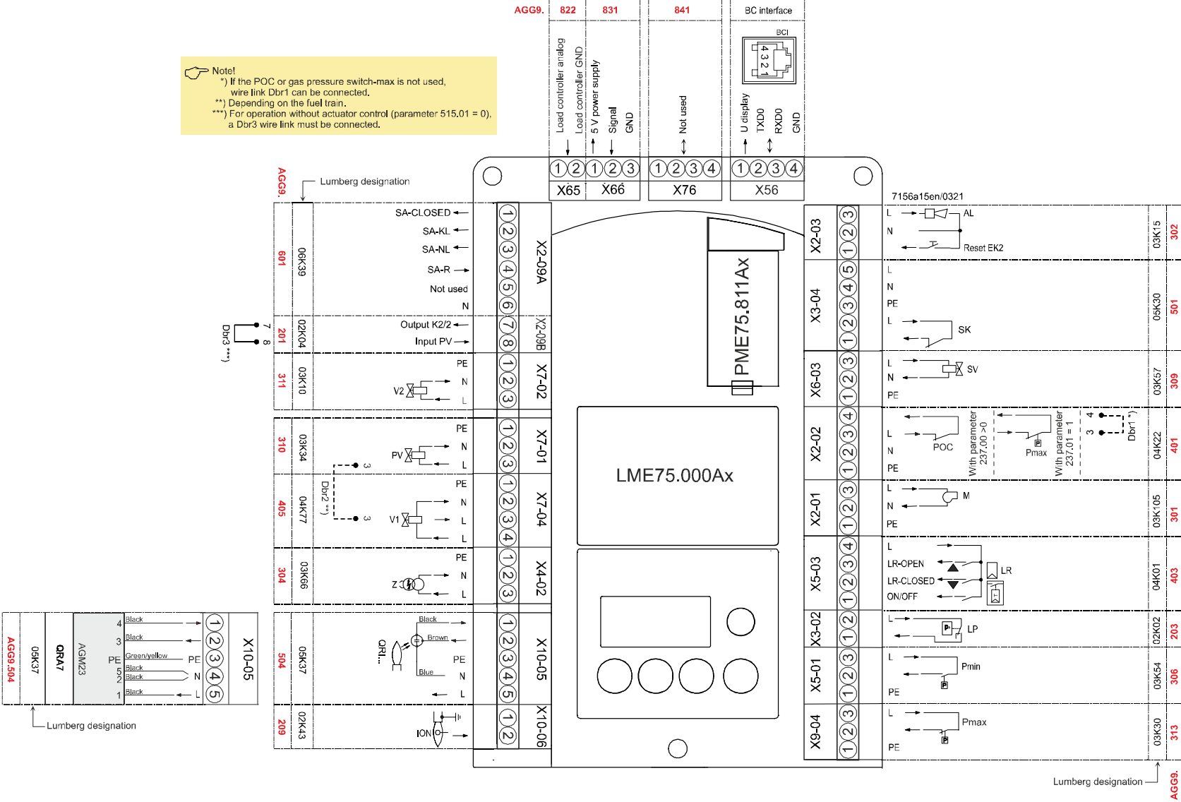
Figure 29: LME75.000Ax: Inputs and outputs / internal connection diagram
