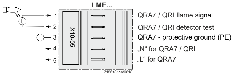
Figure 12: QRA7/QRI terminal X10-05
