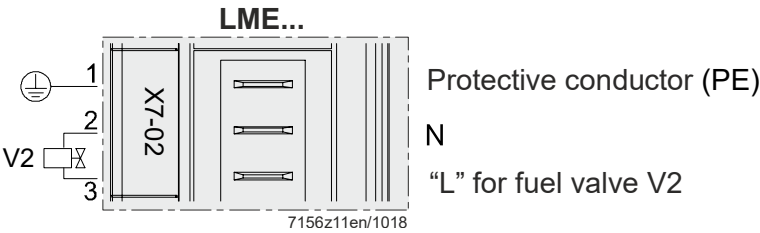
Figure 28: Fuel valve V2 terminal X7-02
