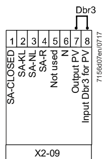
Figure 23: Connection diagram example 2: LME75.000Ax with PME75.811Ax without actuator
