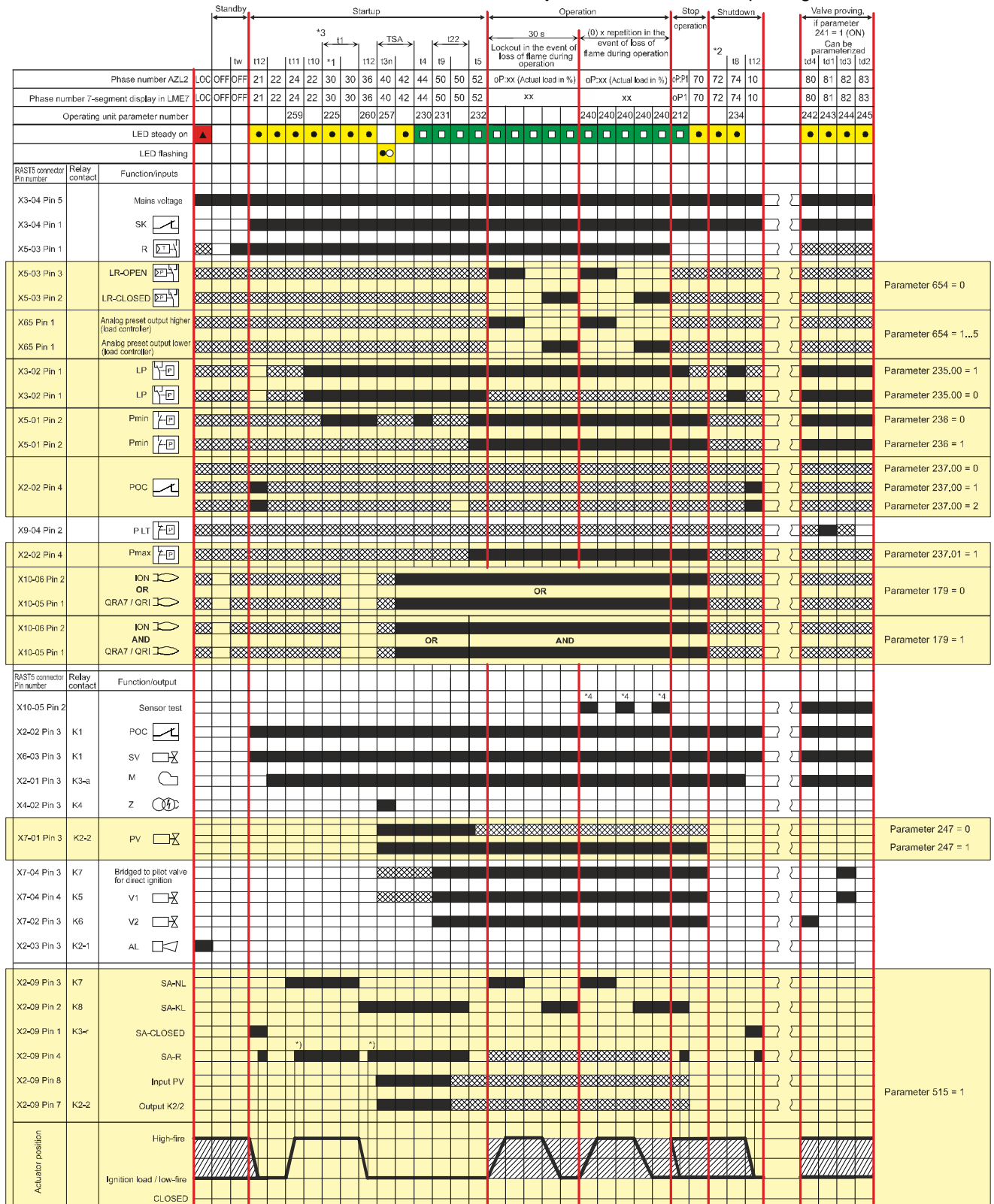
Figure 1: Program sequence for fuel trains G and Gp1 with or without valve proving
