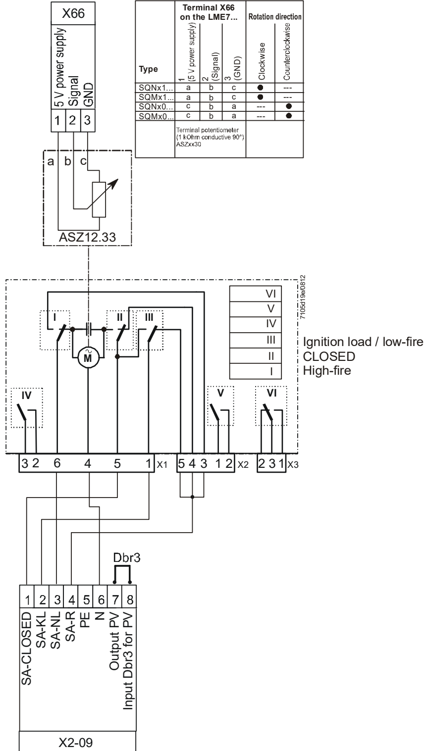
Figure 7: Connection diagram for LME73.000Ax with SQM4
