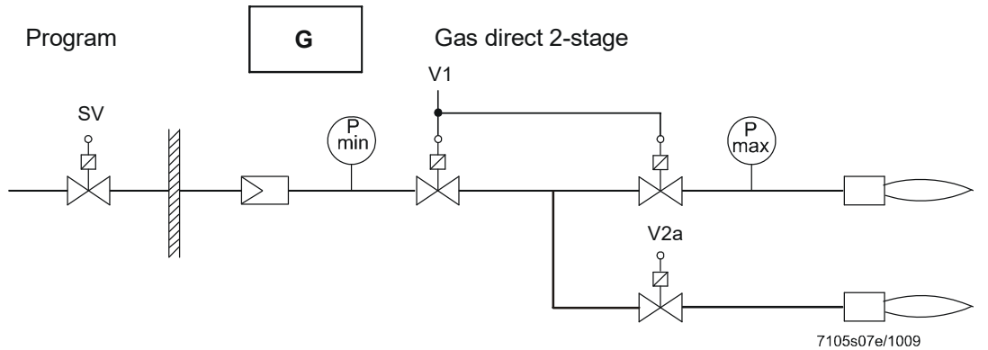
Figure 3: Fuel train gas direct ignition (G), 2-stage
