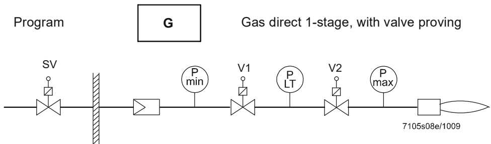
Figure 4: Fuel train gas direct ignition (G), 1-stage, with valve proving
