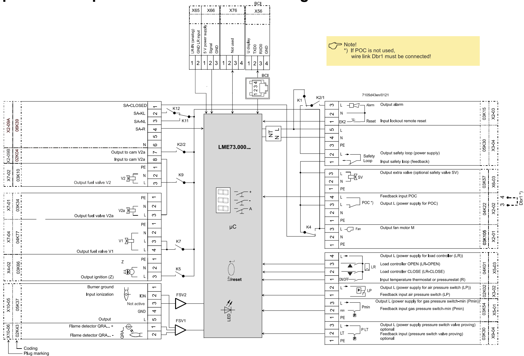
Figure 8: Inputs and outputs / internal connection diagram
